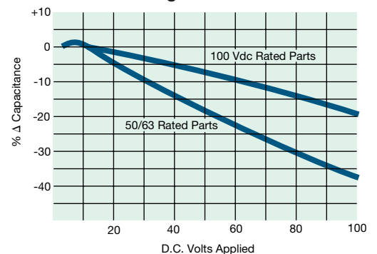
Voltage Coefficient
