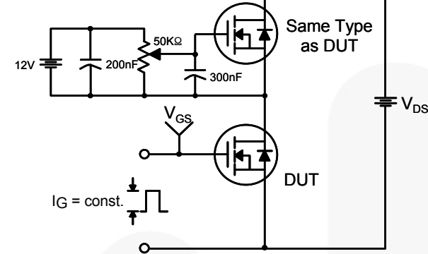
Figure 12. Gate Charge Test Circuit & Waveform
