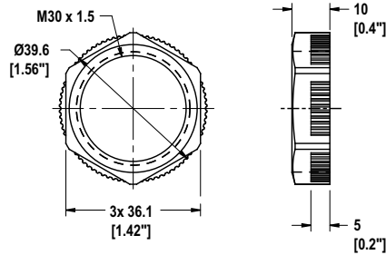
Locknut (included with all models)
