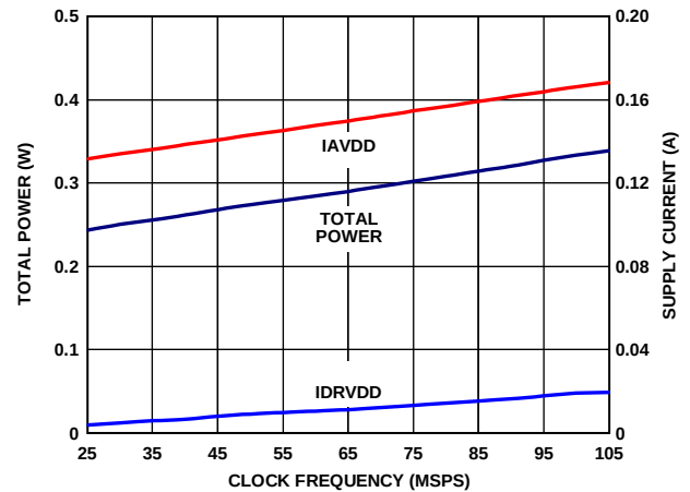
Figure 82. AD9265-105 Power and Current vs. Sample Rate
