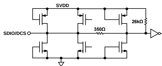
Figure 58. Equivalent SDIO/DCS Circuit
