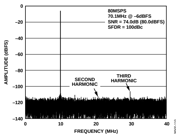
Figure 10. AD9265-80 Single-Tone FFT with f_{IN} = 70.1 MHz @ -6 dBFS with Dither Enabled
