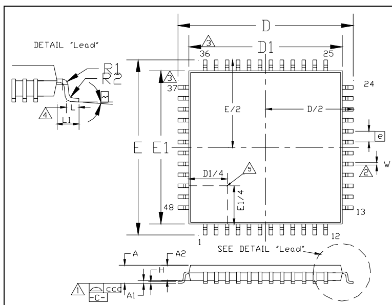
Figure 2 - COM20022I 48 Pin TQFP Package Outline
