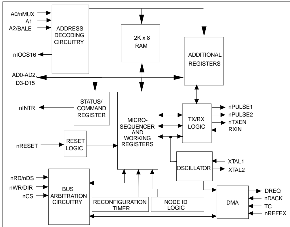
Figure 1 - COM20022I Internal Block Diagram
