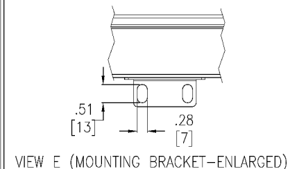
VIEW E (MOUNTING BRACKET-ENLARGED)
