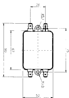
TFN-6, 6-C, 10, 10-C
