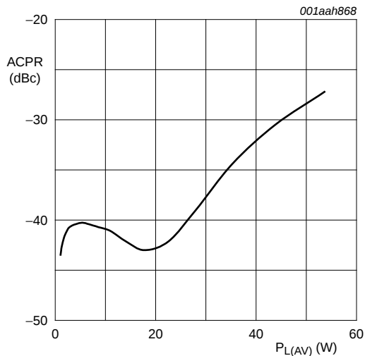
Fig 7. Adjacent power channel ratio as a function of average output power; typical values
