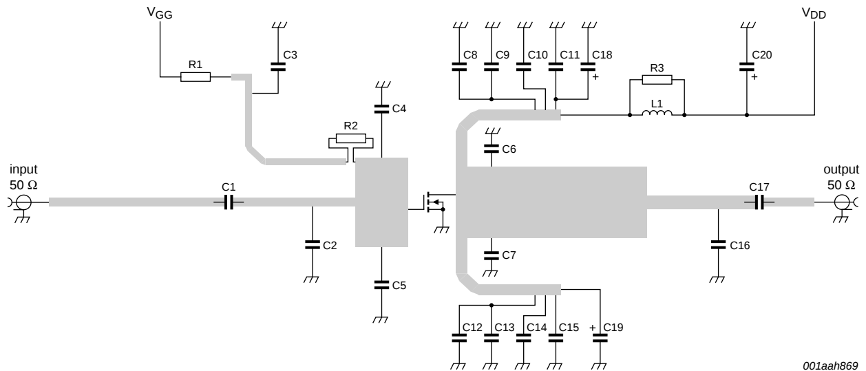
Fig 1. Test circuit for operation at 800 MHz
