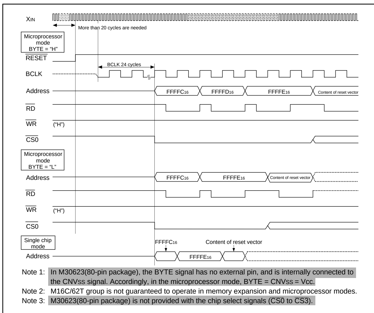
Figure 1.6.2. Reset sequence
