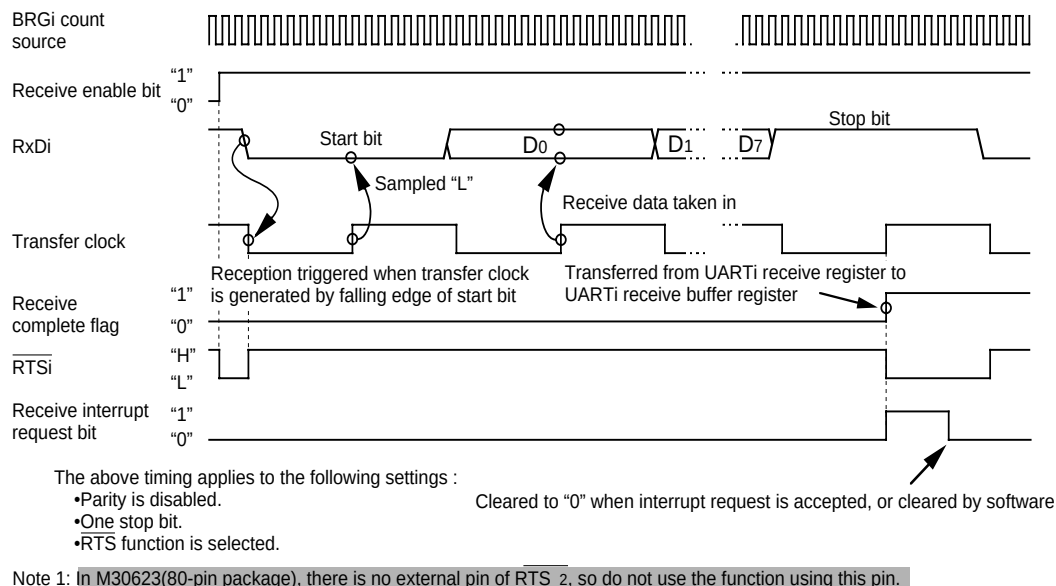
Figure 1.19.17. Typical receive timing in UART mode
