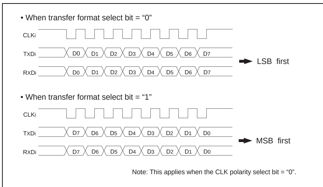
Figure 1.19.12. Transfer format
