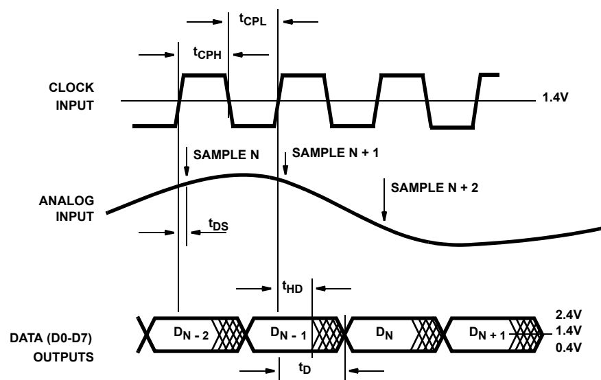
FIGURE 1. INPUT-TO-OUTPUT TIMING
