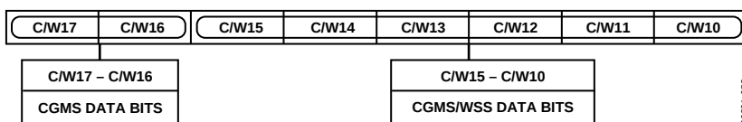
Figure 52. CGMS_WSS Register 1
