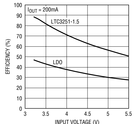
1.5V Efficiency vs Input Voltage (Burst Mode Operation)
