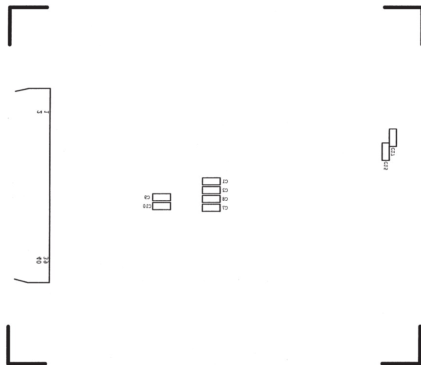
Figure 30. Silkscreen Layer—Bottom
