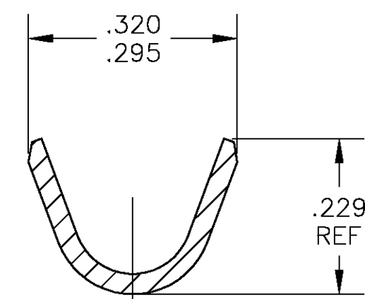
SECTION Y-Y
