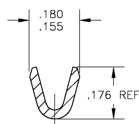
SECTION X-X
