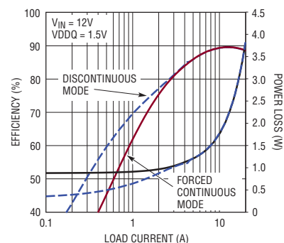
Efficiency/Power Loss VDDR Channel 1
