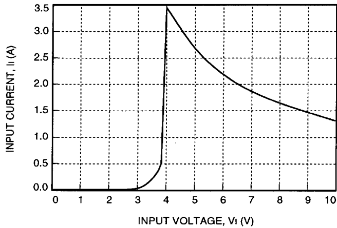
Figure 1. MH010-Series Typical Input Characteristic with I_o = I_{o, \max} ; T_c = 25^\circ\text{C}
