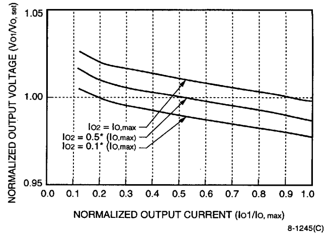
Figure 3. MH010BK, CL Typical Regulation: V_o vs. I_o for V_{IN} = 5\text{ V} , T_c = 25^\circ\text{C}
