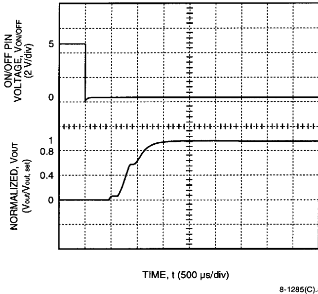
Figure 9. Typical Output Voltage Start-Up When Remote On/Off Is Enabled; I_o = 80\% of I_{o, \max}
