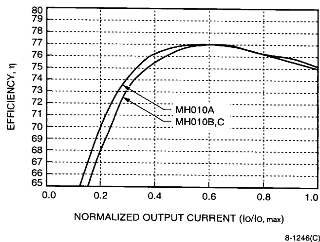
Figure 7. MH010A, B, C Typical Converter Efficiency as a Function of Output Current with V_I = 5\text{ V} and T_A = 25\text{ }^{\circ}\text{C}
