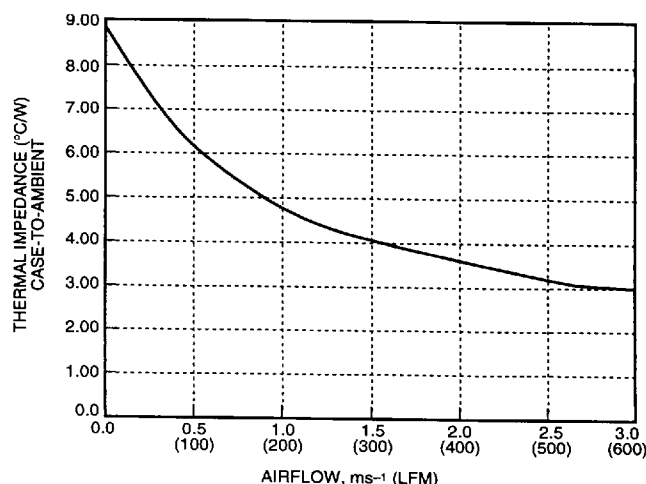
Figure 17. MH010A, B, C Case-to-Ambient Thermal Impedance
