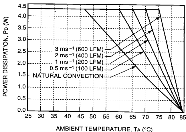
Figure 16. Convection Derating Power Derating with No Heat Sink; Either Orientation
