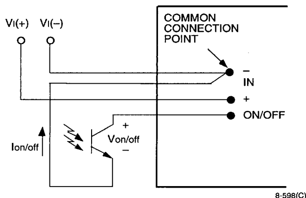
Figure 14. Remote On/Off Circuitry
