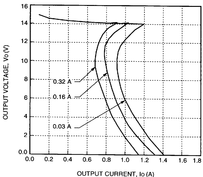
Figure 6. MH010CL Typical Output Characteristics with V_{IN} = 5\text{ V} , T_A = 25\text{ }^{\circ}\text{C}
