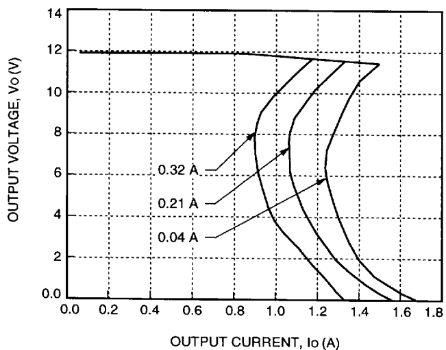
Figure 5. MH010BK Typical Output Characteristics with V_{IN} = 5\text{ V} , T_A = 25\text{ }^{\circ}\text{C}
