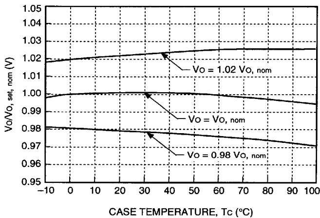
Figure 2. MH010-Series Typical Output Voltage Variation Over Operating Case Temperature
