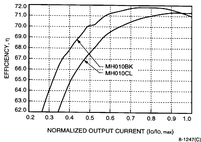
Figure 8. MH010BK, CL Typical Converter Efficiency as a Function of Output Current with V_I = 5\text{ V} and T_A = 25\text{ }^{\circ}\text{C}
