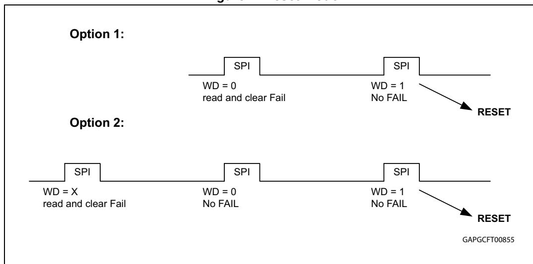
Figure 7. Reset mode
