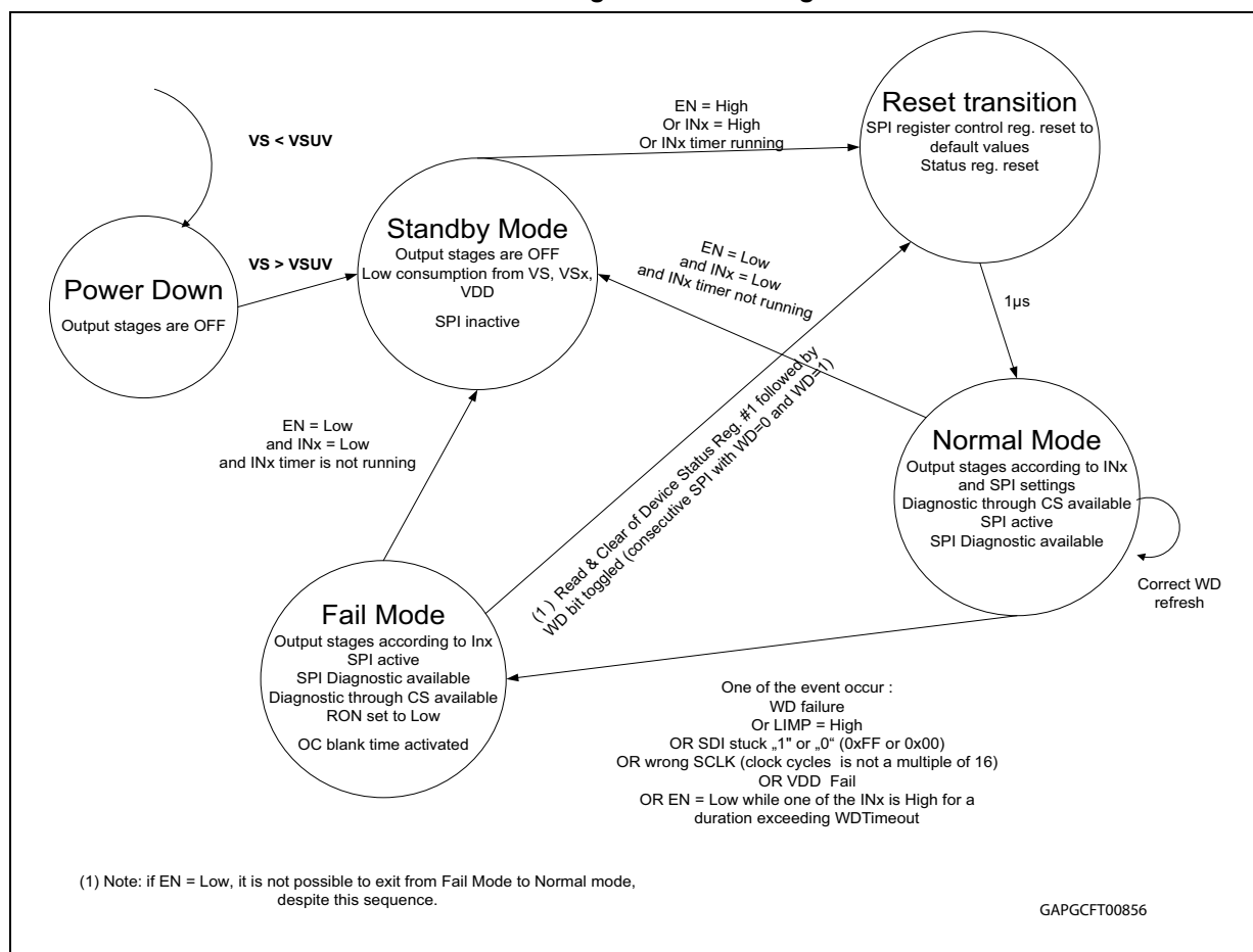
Figure 4. State diagram
