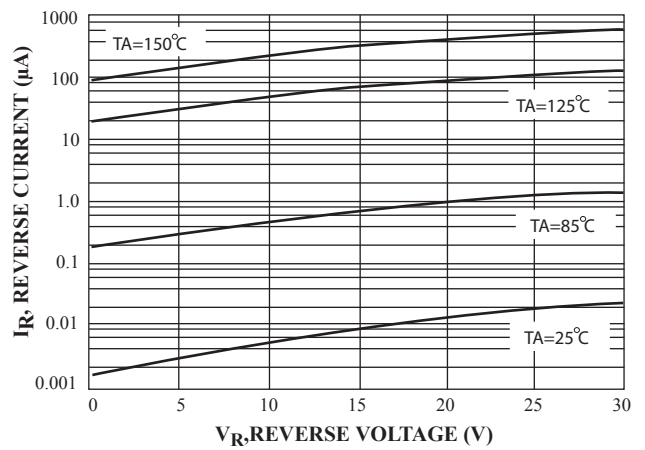
FIG.3 Leakage Current
