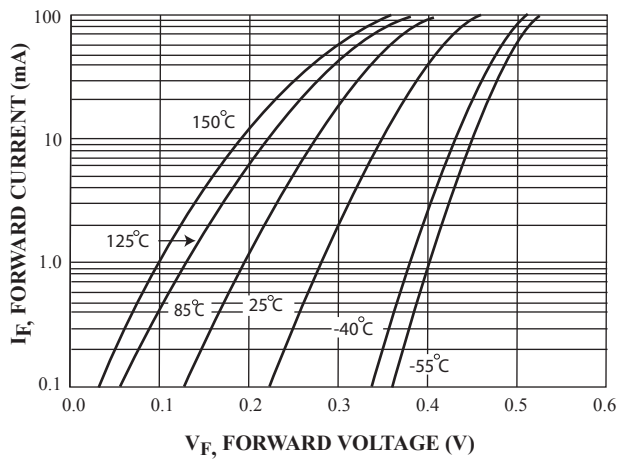
FIG.2 Forward Voltage
