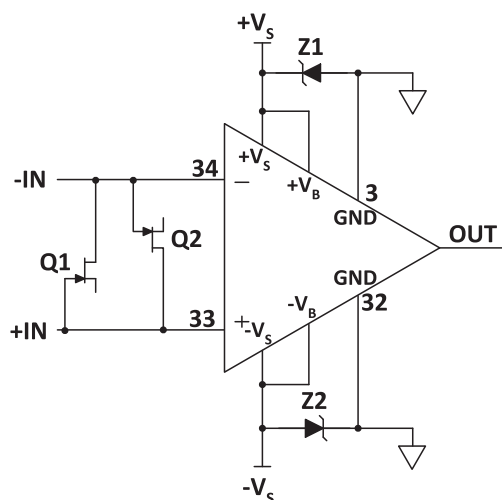
Figure 17: Overvoltage Protection
