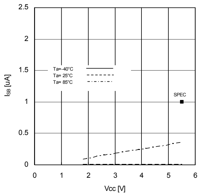
Figure 18. Standby Current vs Supply Voltage
