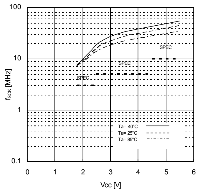
Figure 19. SCK Frequency vs Supply Voltage
