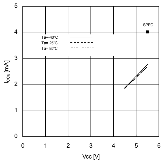
Figure 17. Supply Current (Read) vs Supply Voltage (fSCK=10MHz)
