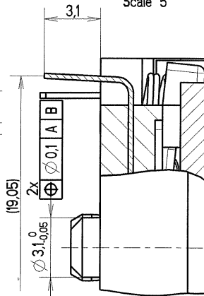
DETAIL A Scale 5
