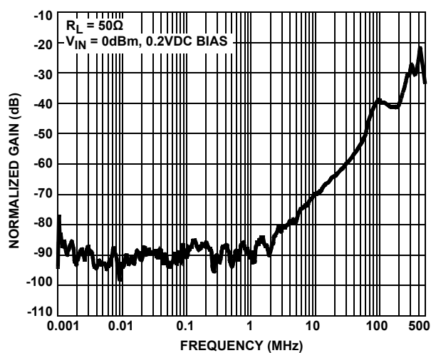
FIGURE 26. CROSSTALK
