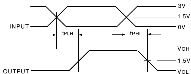
Pulse Skew - t_{sk(p)}
