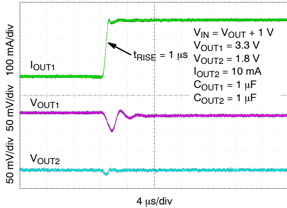
Figure 36. Load Transient Response – 1.8 V – Rising Edge, I_{OUT1} = 100\text{ }\mu\text{A} to 300 mA
