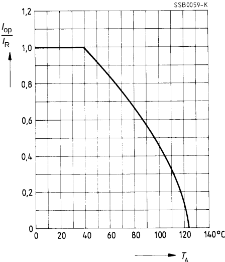
Current derating I_{\text{op}}/I_{\text{R}} versus ambient temperature T_{\text{A}} (Rated temperature T_{\text{R}} = 40^\circ\text{C} )
