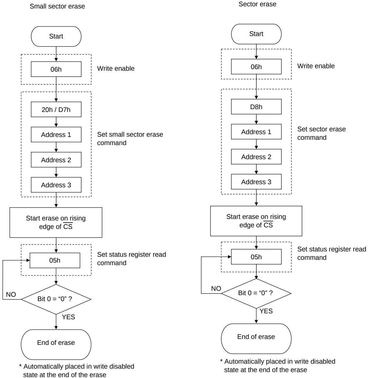
Figure 21 Erase Flowcharts
