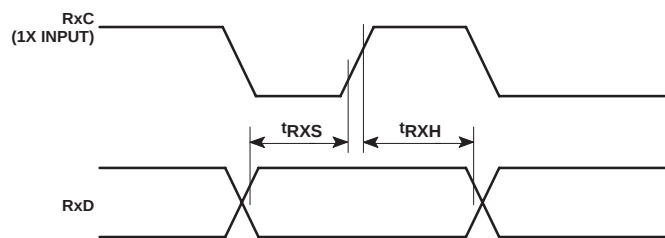
Figure 11. Receive Timing
