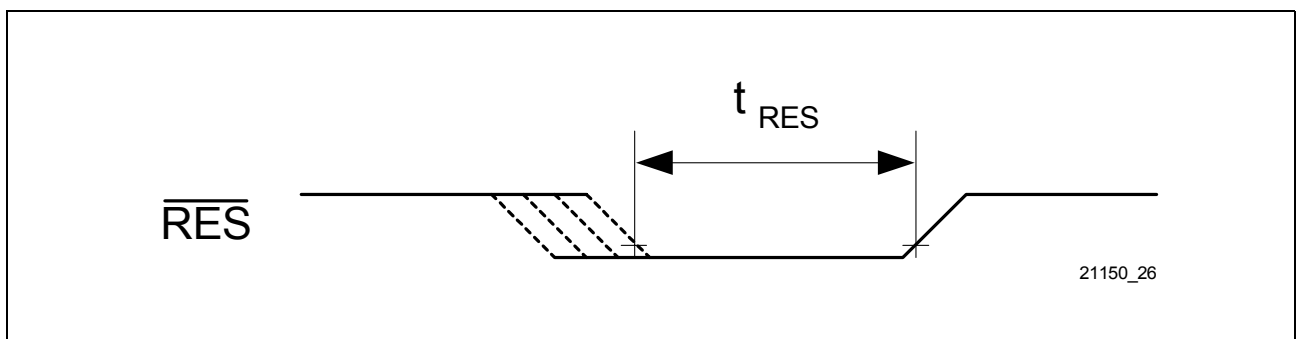
Figure 96 Reset Signal \overline{\text{RES}}
