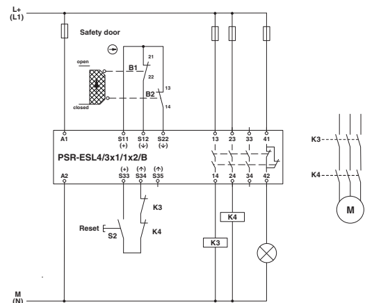
Figure 7 Two-channel safety door monitoring without cross-circuit detection
