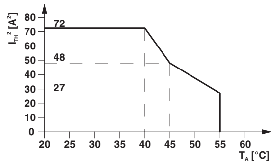
Figure 2 Derating curve
