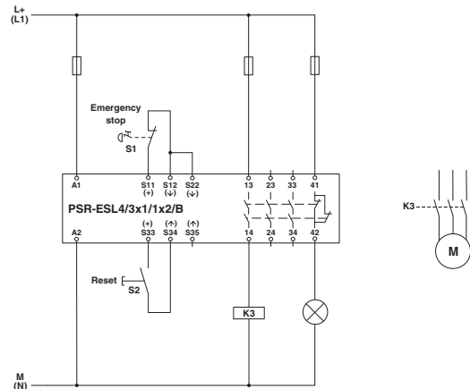
Figure 6 Single-channel emergency stop circuit with monitored reset button
