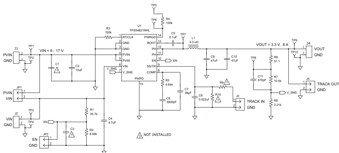
Figure 4-1. TPS54821EVM-049 Schematic
