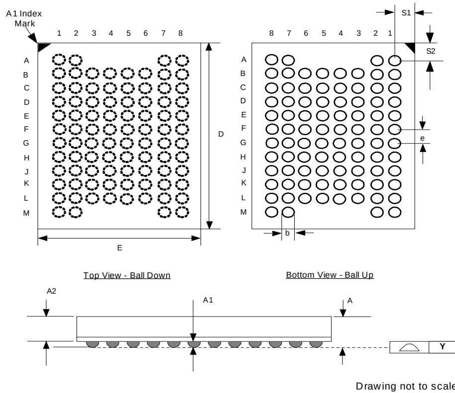
Figure 5. 512-Mbit, 88-ball (80 active) QUAD+ SCSP Specifications (8x11x1.2 mm)
