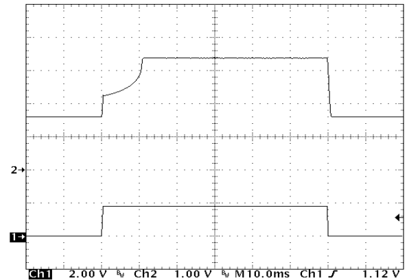
Upper Trace: Output Voltage Waveform, 2.0 V/Division Lower Trace: Shutdown Pin Waveform, 1.0 V/Division
