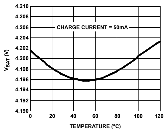
FIGURE 5. CHARGER OUTPUT VOLTAGE vs TEMPERATURE
