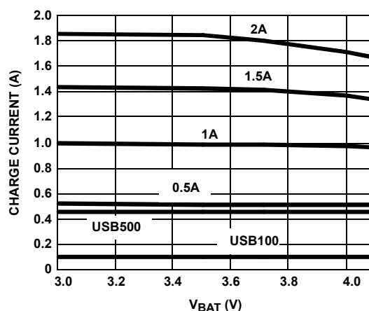
FIGURE 7. CHARGE CURRENT vs OUTPUT VOLTAGE
