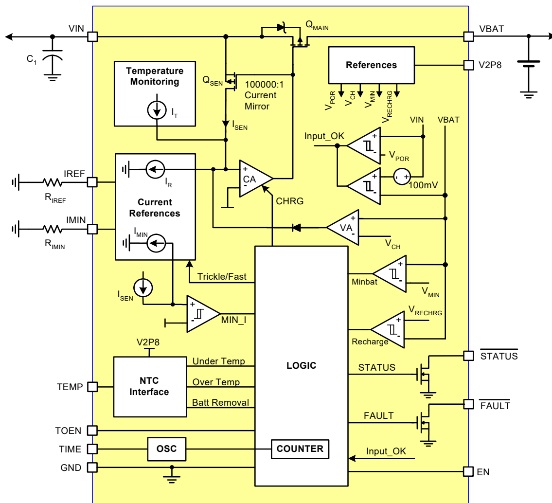
FIGURE 3. BLOCK PROGRAM
