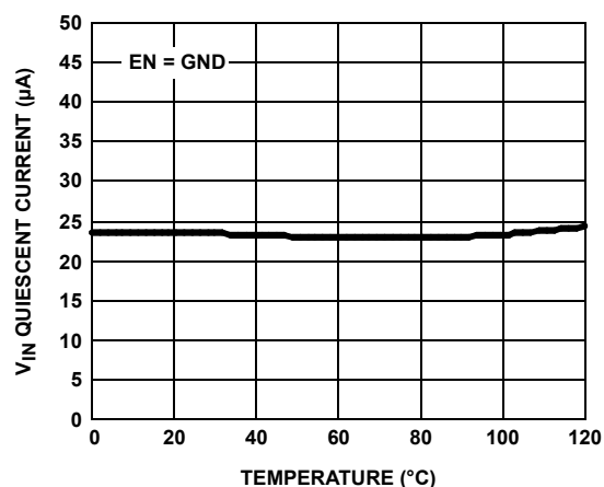
FIGURE 15. INPUT QUIESCENT CURRENT vs TEMPERATURE
