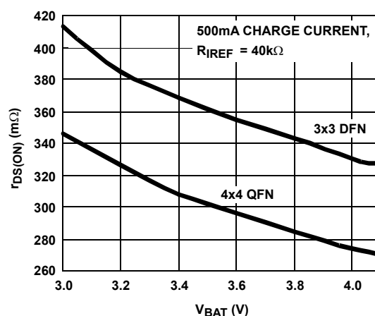
FIGURE 13. r_{DS(ON)} vs OUTPUT VOLTAGE USING CURRENT LIMITED ADAPTERS
