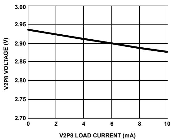
FIGURE 11. V2P8 OUTPUT vs ITS LOAD CURRENT
