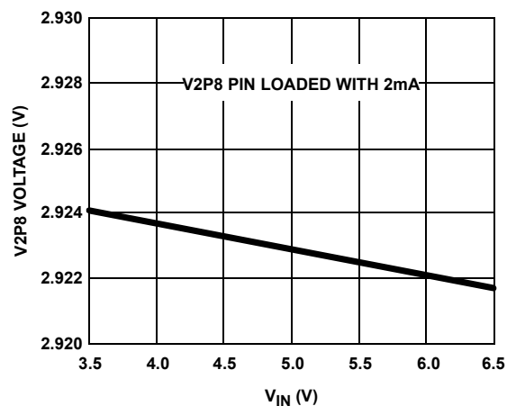
FIGURE 10. V2P8 OUTPUT vs INPUT VOLTAGE
