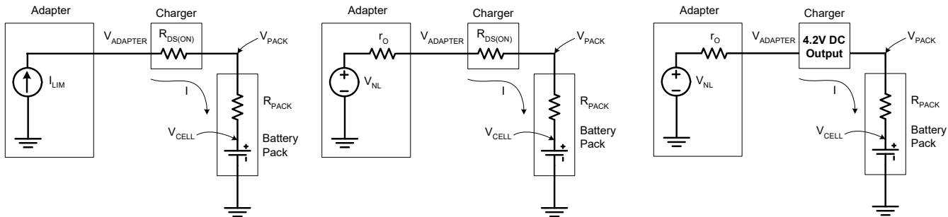
FIGURE 27A. THE EQUIVALENT CIRCUIT IN THE CONSTANT CURRENT REGION
