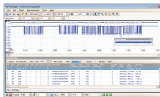
Serial decoding
