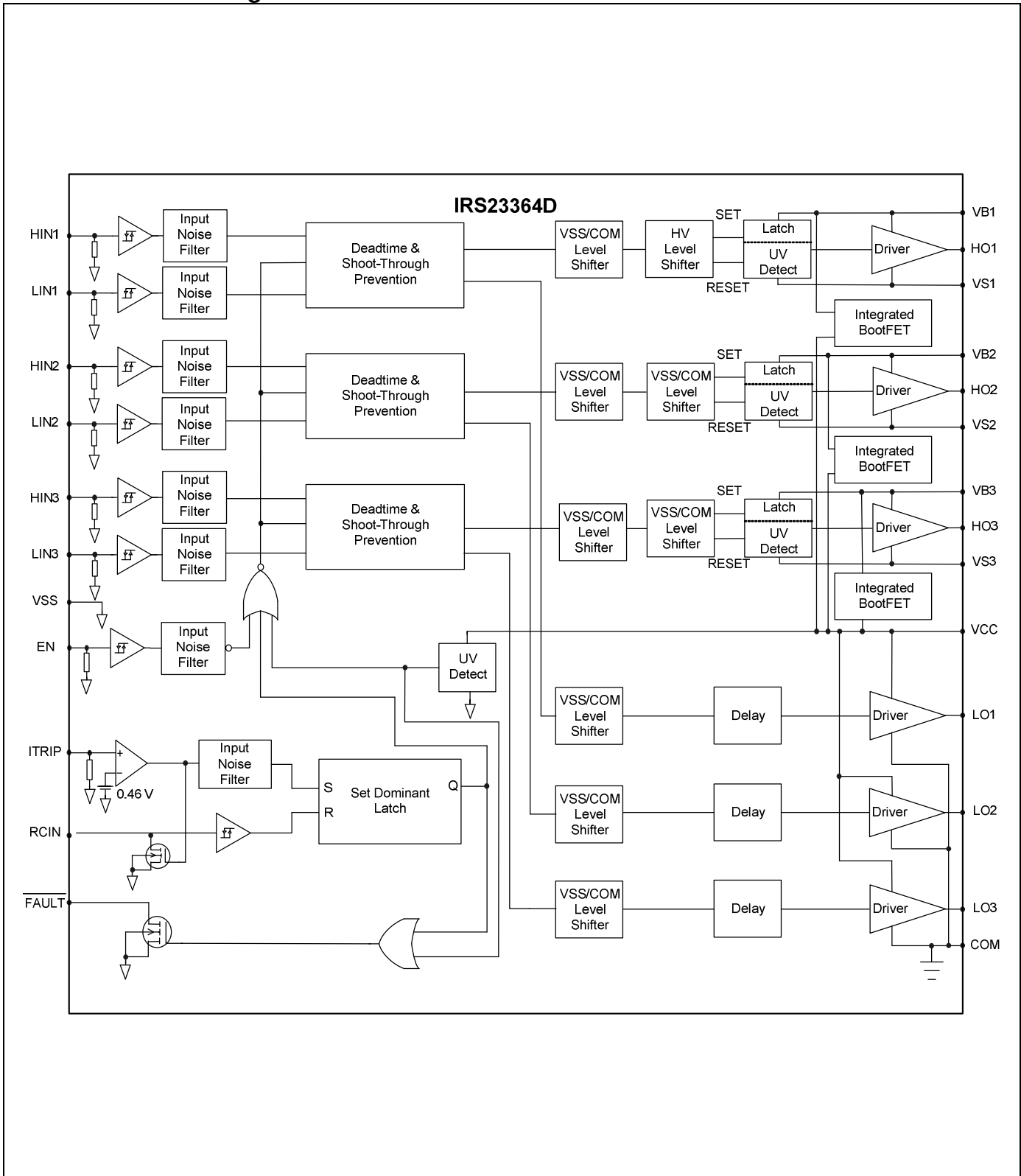
Functional Block Diagram: IRS23364D
