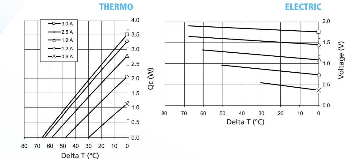
Performance Curves at T_h = 50^\circ\text{C}
