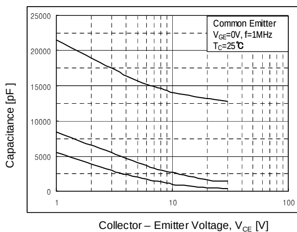
Fig 15. Capacitance characteristic
