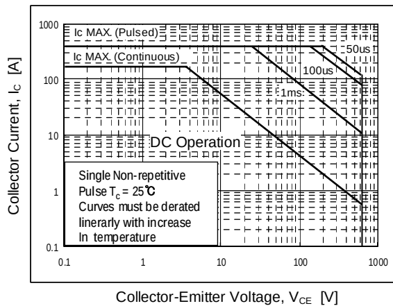
Fig11. SOA characteristics
