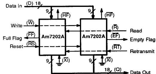
Figure 13. Width-Expansion to Form a 1,024x18 FIFO
