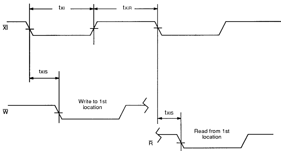
Figure 11. 1st Clock Pulse Delay from \overline{X1}
