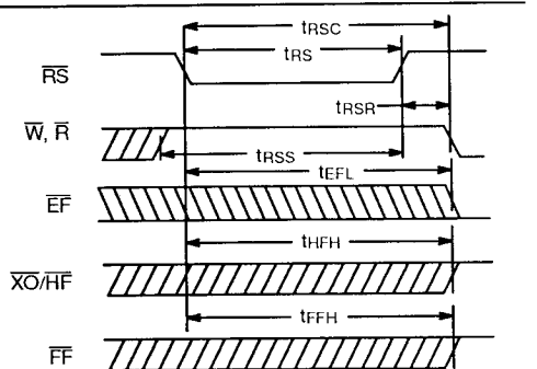
Figure 2. Reset Timing
