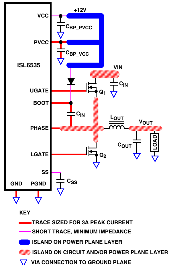
FIGURE 5. PRINTED CIRCUIT BOARD POWER PLANES AND ISLANDS
