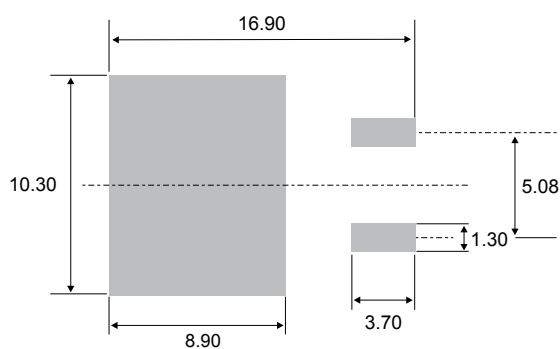
Figure 13. D 2 PAK recommended footprint (dimensions are in mm)
