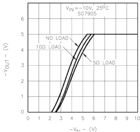
Figure 7 – Dropout Characteristics
