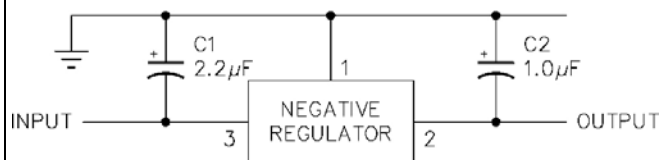
Figure 9 – Fixed Output Regulator
