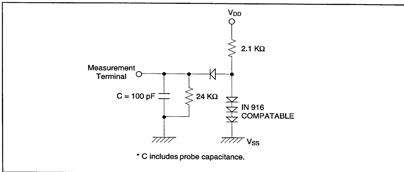
Figure 38. Measurement circuit
