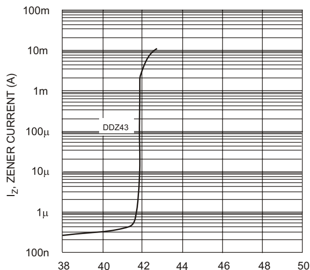
Fig. 9 Typical Reverse Characteristics, DDZ43
