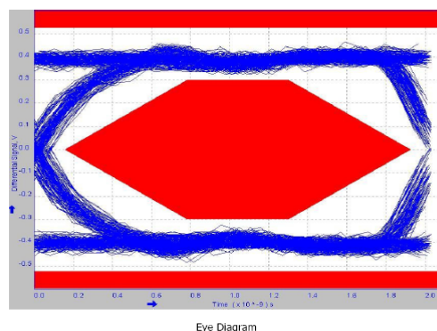
Fig. 4:Eye Diagram example (480MHz) computed from the USB-IF test pattern during USB2.0 compliance verification of an existing HOST PHY ASIC clocked at 48MHz by PCS3P73U00A.
