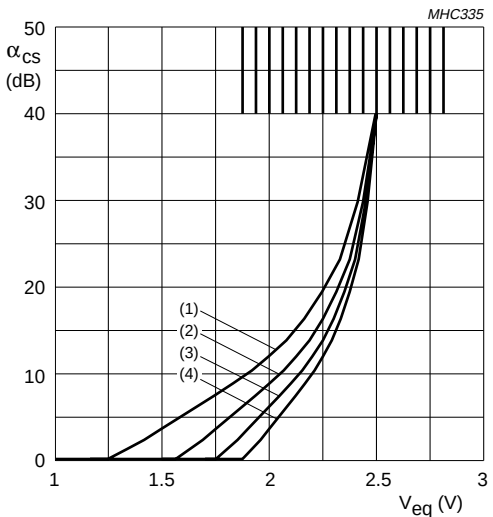
SST[3:0] = 1010 (1) SSL[1:0] = 00 = 38 dB/V. (2) SSL[1:0] = 01 = 51 dB/V. (3) SSL[1:0] = 10 = 63 dB/V. (4) SSL[1:0] = 11 = 72 dB/V.
