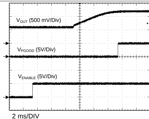
Figure 18. Start-up With Prebiased Output
