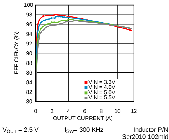
Figure 3. Efficiency
