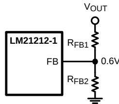
Figure 27. Setting V_{OUT}
