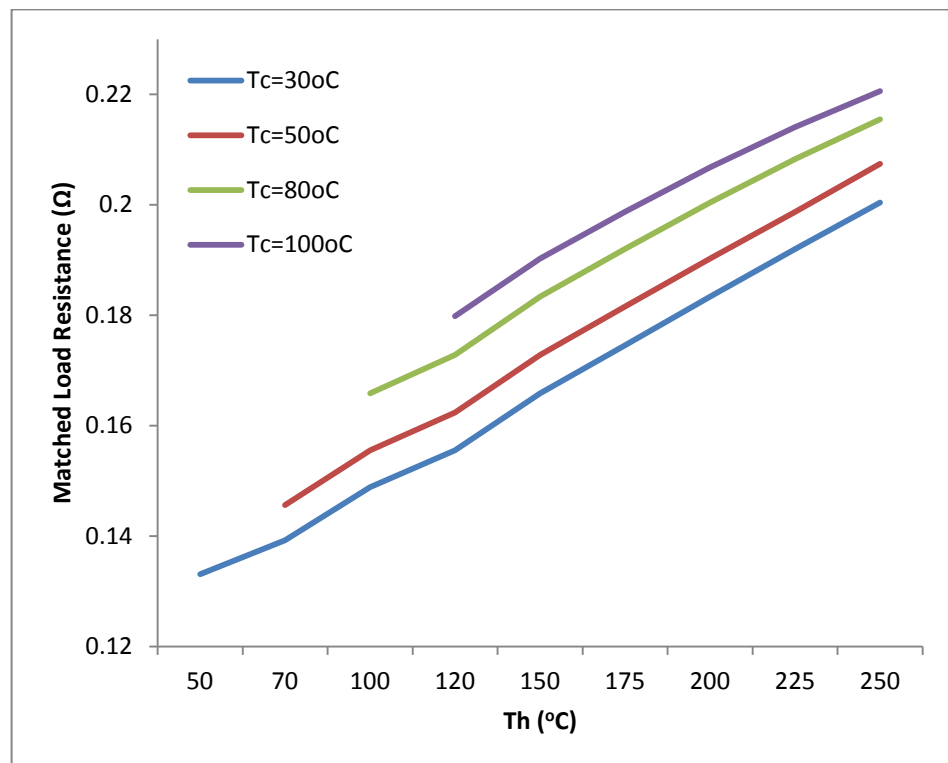
Matched Load Resistance v. Hot side for various fixed cold sides
