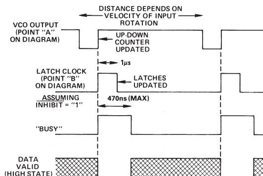
Figure 1. Timing Diagram
