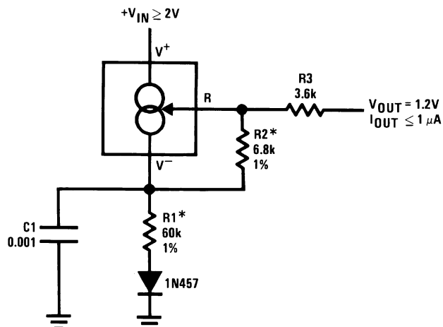
Figure 25. 1.2V Reference Operates on 10 µA and 2V
