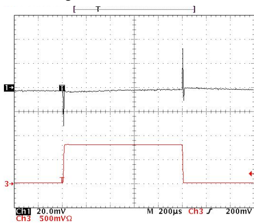
Figure 17. Load transient
