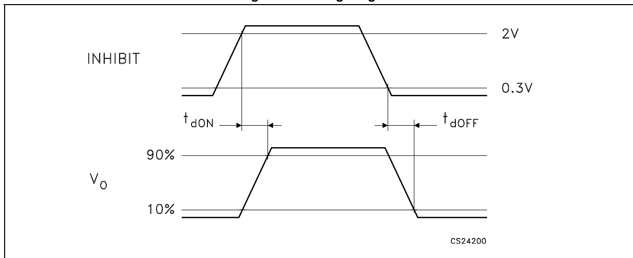
Figure 4. Timing diagram
