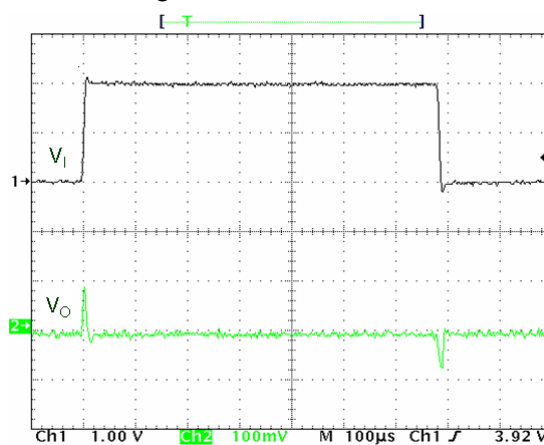
Figure 18. Line transient
